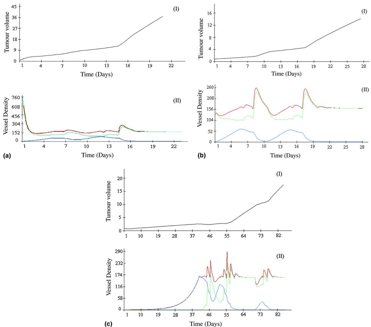
Fig. 2. Simulations of the vascular tumour growth model showing relatively fast (2a), moderate (2b) and slow (2c) growing tumours. Tumour volume ( \text{mm}^3 ; I) and vessel density (VD) ( \mu\text{m}^3 ; II) as calculated by the model, using the estimated average spheroid parameters, varying only in initial VD, were plotted as a function of time (days). The total VD, mature vessel density (MatVD), and immature vessel density (ImmVD) are denoted by red (top curve), green (middle curve) and blue (bottom curve), respectively. Note the difference in dimensions between the biological range of VD, as calculated by the model in this figure, and the VD dimensions appearing in Figs. 4 and 5, which reflect magnetic resonance imaging (MRI) procedures.
